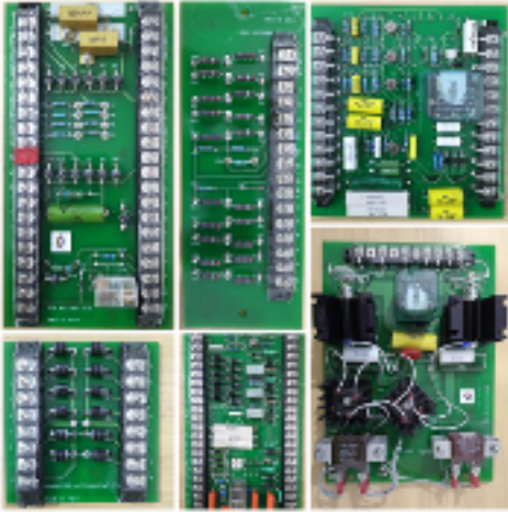
SCR PCBs
